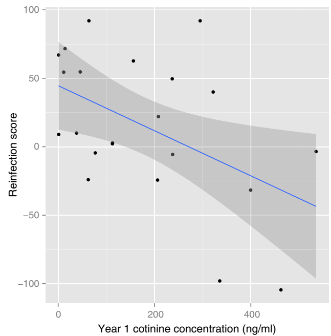
Fig. 3. Scatterplot of reinfection scores vs. year 1 cotinine concentration. Reinfestation score = mean year 2 worm burden (s7–s9) minus mean year 1 worm burden (s4–s6). Line fit by linear regression. Shading represents \pm 2 SE.
