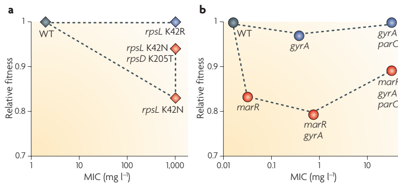
Figure 3 | Relationship between antibiotic resistance and bacterial fitness.
